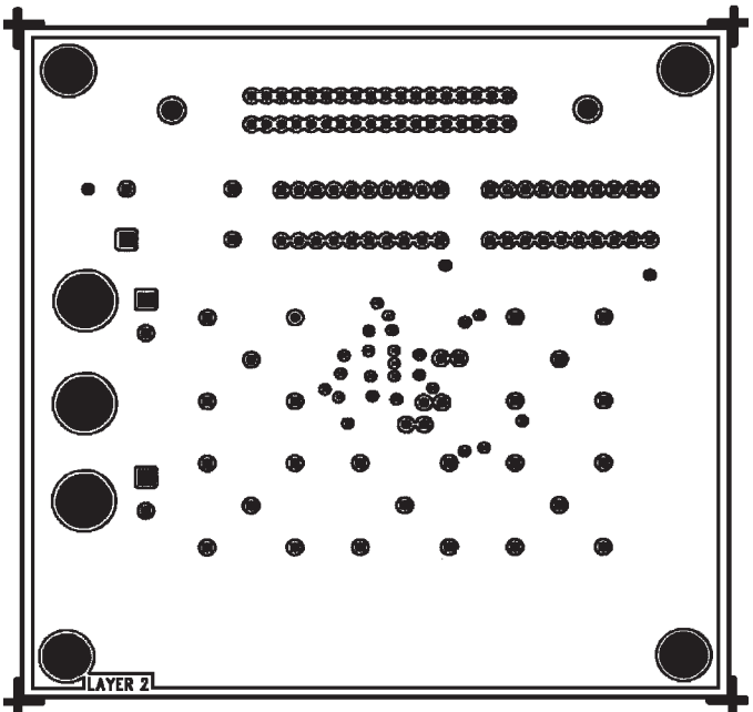
25c. CGPCB Power Plane
