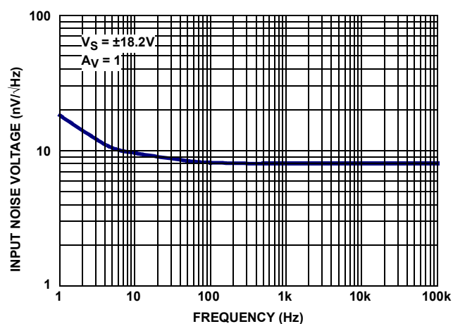
FIGURE 36. INPUT NOISE VOLTAGE SPECTRAL DENSITY
