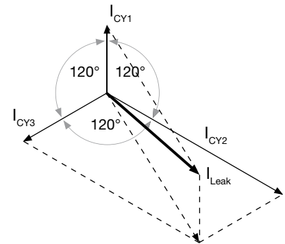
Figure 6: Determination of resultant leakage current at three phase filters
