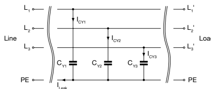
Figure 5: Y capacitors in a three phase filter
