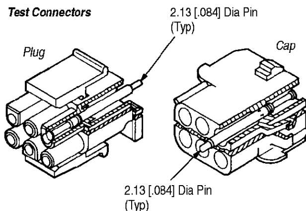
TEST CONNECTORS •
