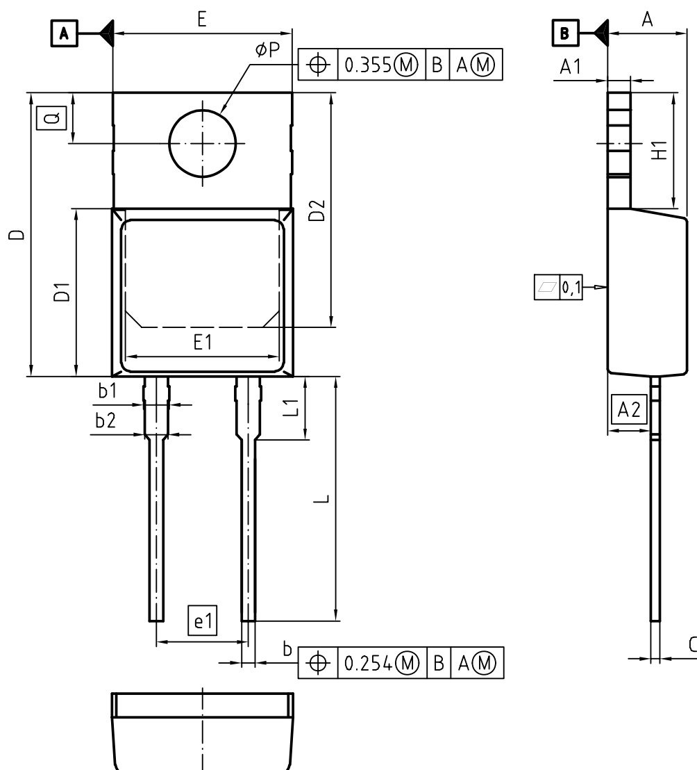
TO-220-2
