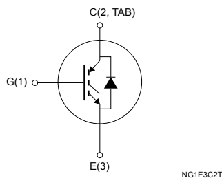
TO-247
