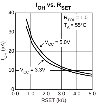
Figure 1. DC Response
