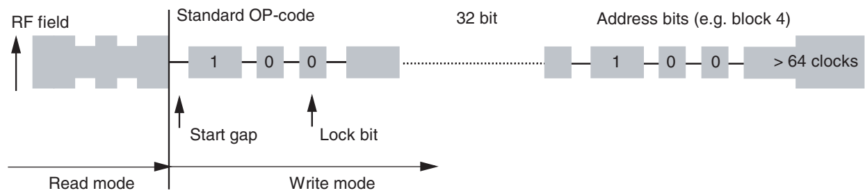
Figure 8-1. Write Protocol
