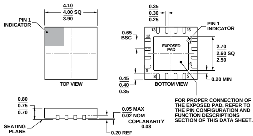
Figure 56. 16-Lead Lead Frame Chip Scale Package [LFCSP_WQ] 4 mm × 4 mm Body, Very Very Thin Quad (CP-16-17)
