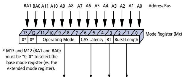
Figure 5: Mode Register Definition Diagram
