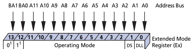
Figure 7: Extended Mode Register Definition Diagram
