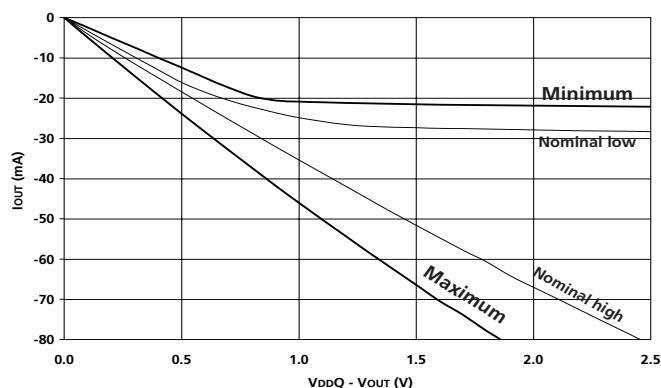
Figure 12: Reduced Output Pull-Up Characteristics
