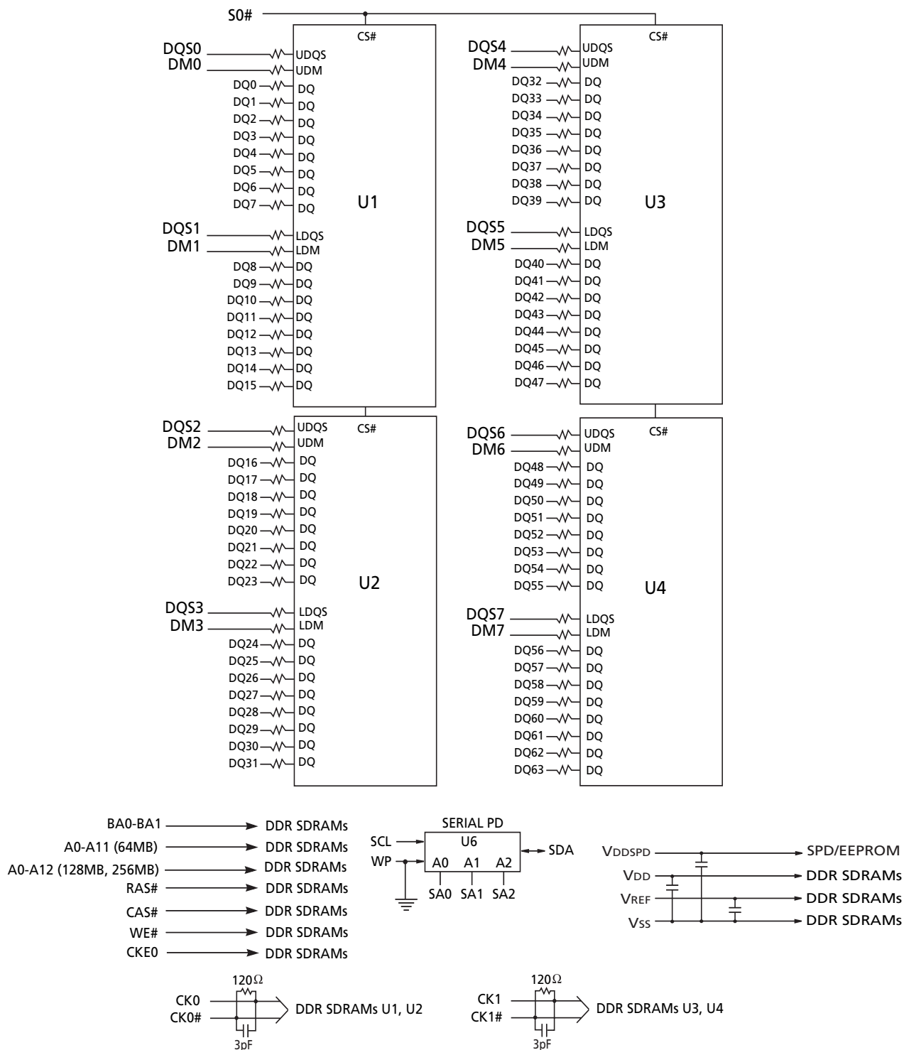
Figure 3: Functional Block Diagram – 64MB
