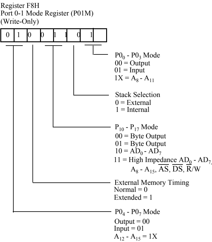
Figure 5-27. Port 0/1 Reset
