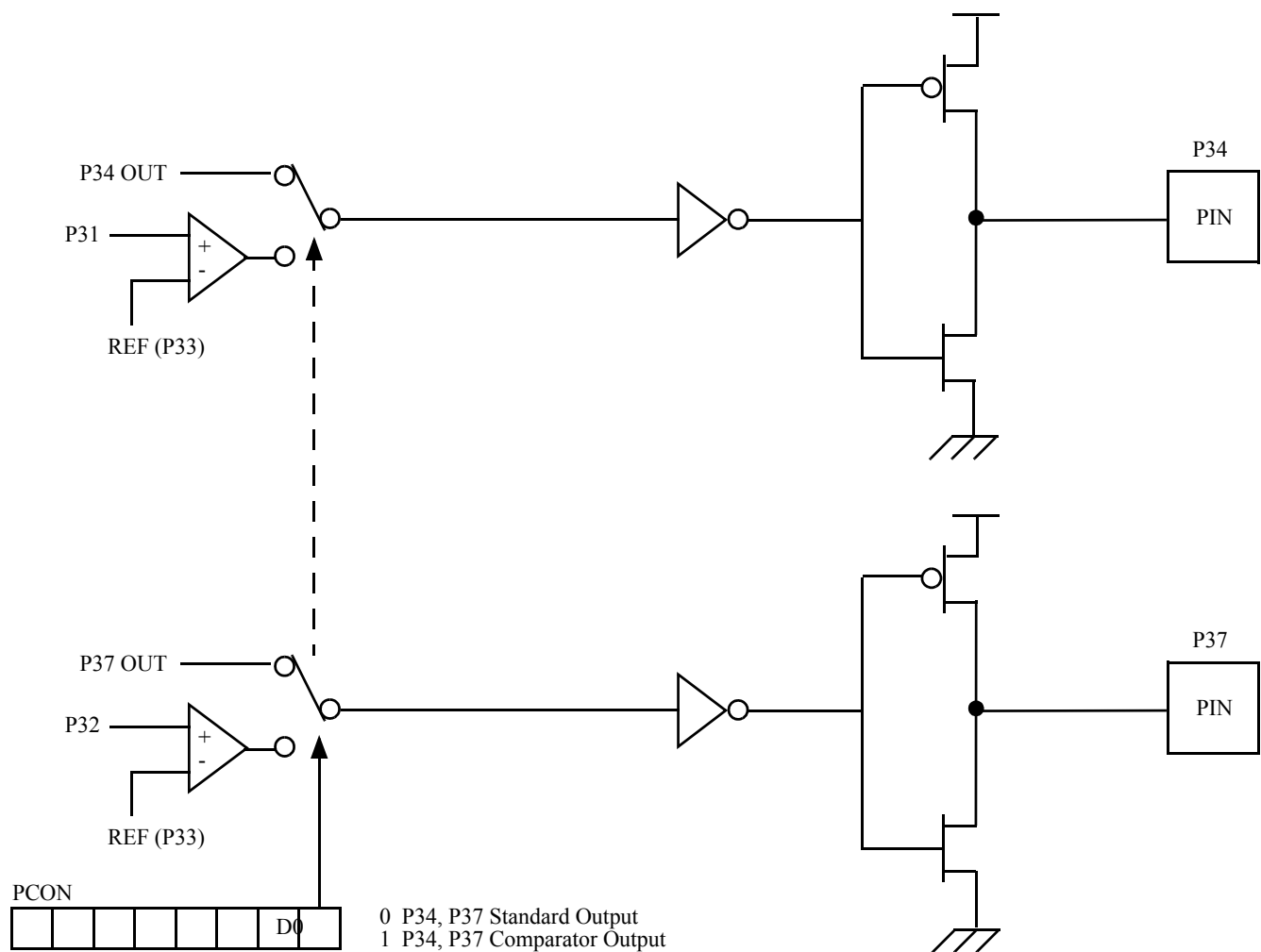
Figure 5-33. Port 3 Configuration
