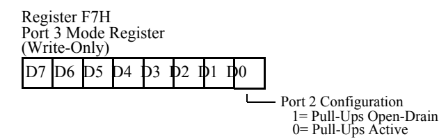
Figure 5-34. Port 2 Configuration
