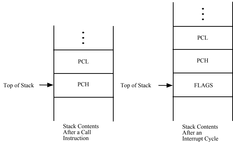
Figure 2-10. Stack Operations
