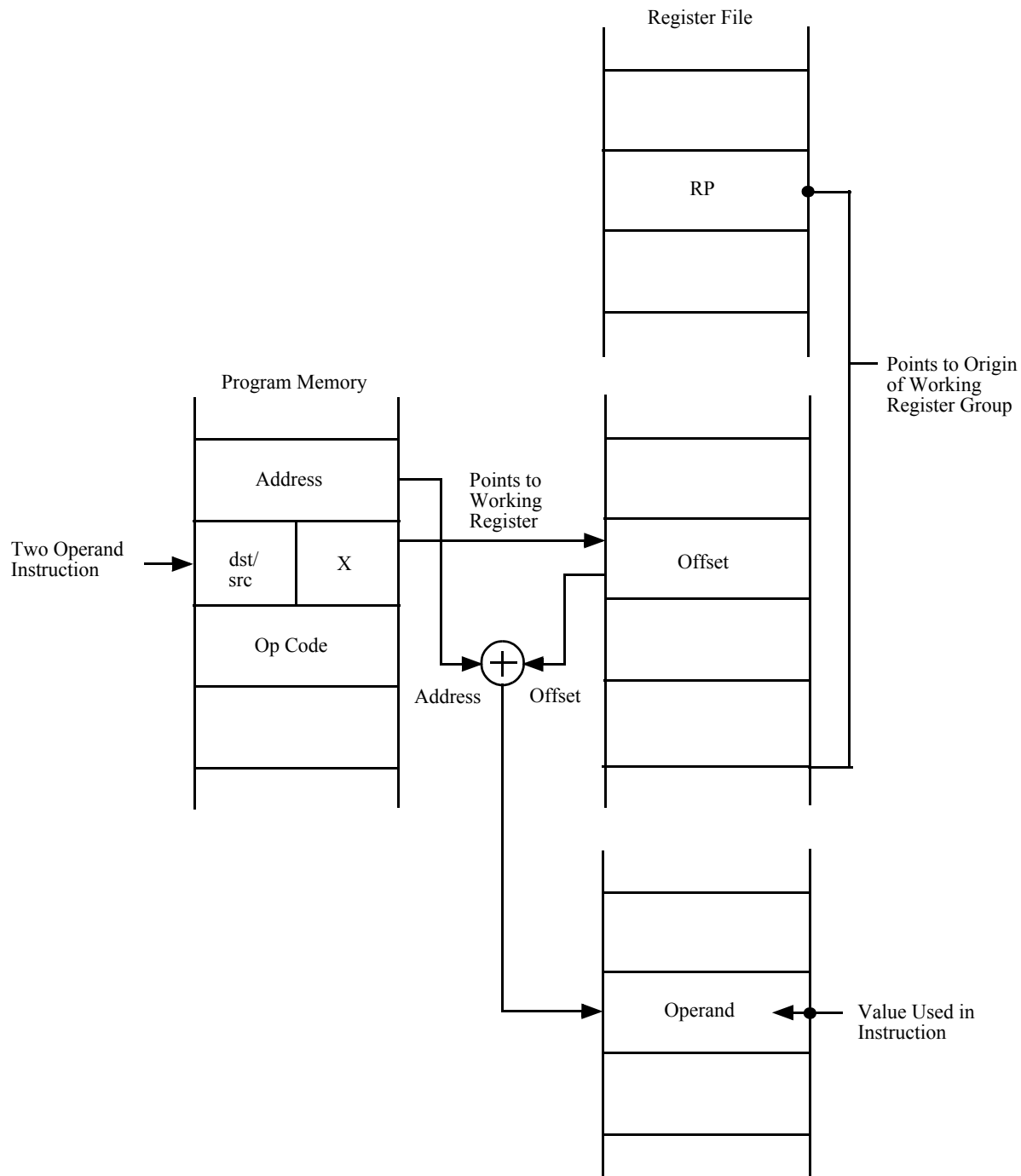
Figure 11-5. Indexed Register Addressing
