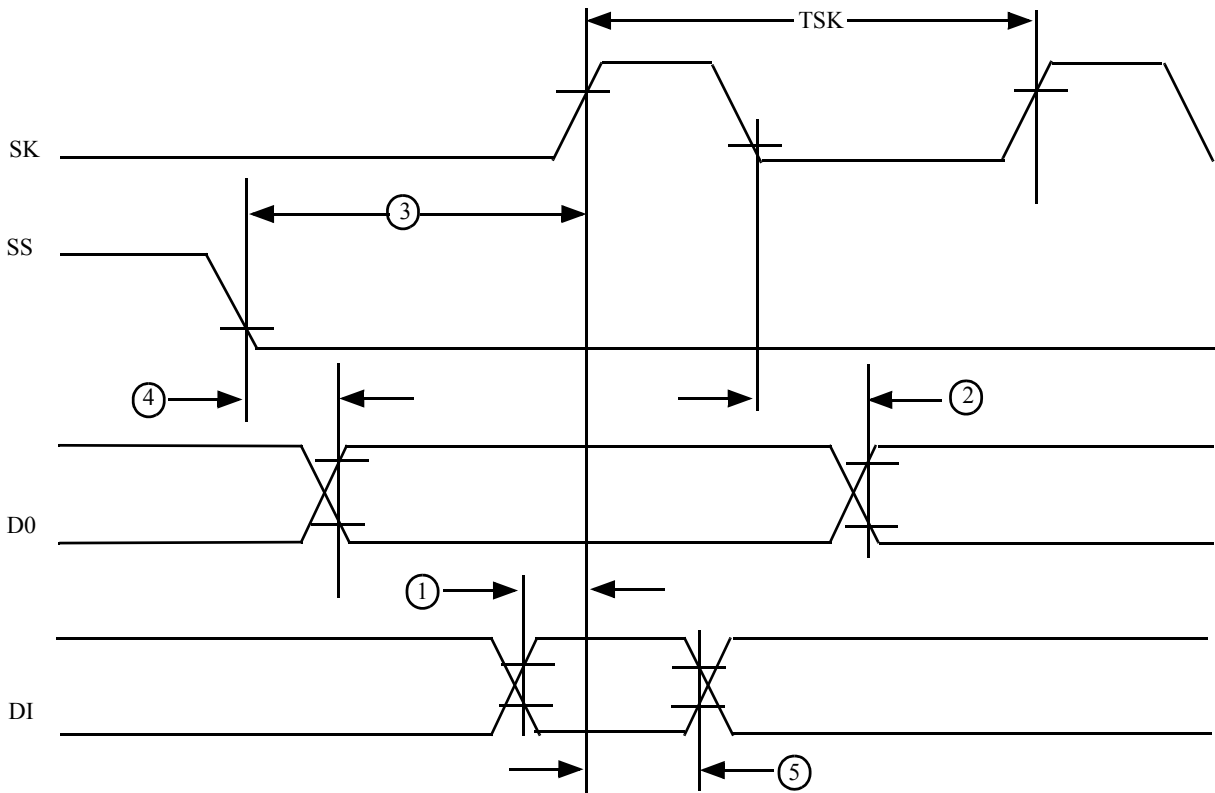
Figure 9-14. SPI Timing
