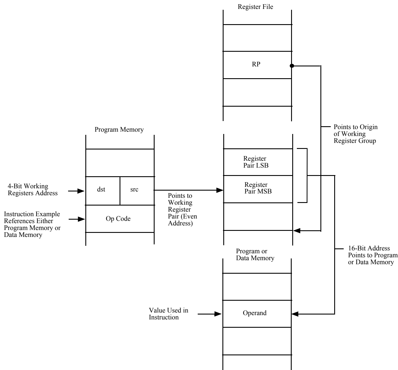
Figure 11-4. Indirect Register Addressing to Program or Data Memory
