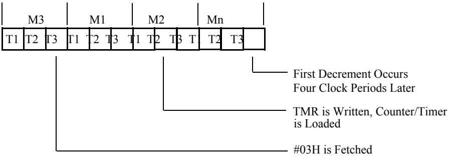
Figure 6-8. Counting Modes
