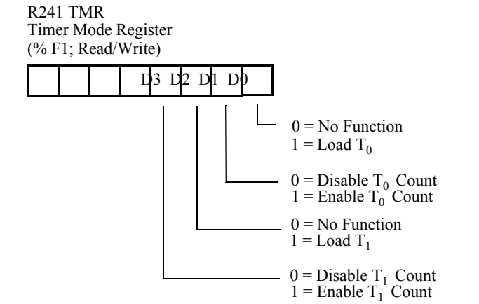
Figure 6-6. Timer Mode Register
