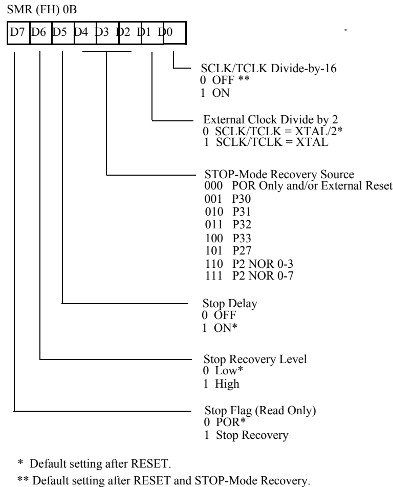
Figure 8-1. STOP-Mode Recovery Register (Write-Only Except Bit D7, Which Is Read-Only)
