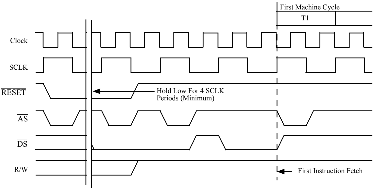
Figure 4-1. Reset Timing
