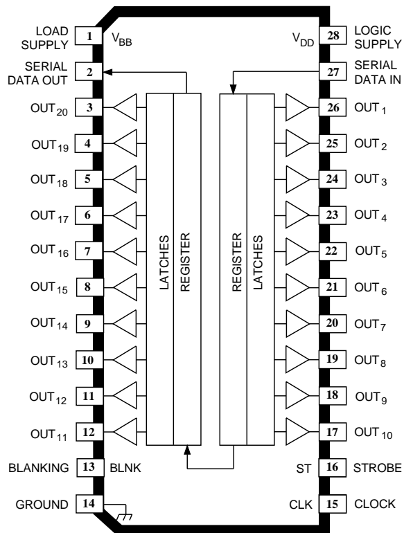
A6812xLW (SOIC)
