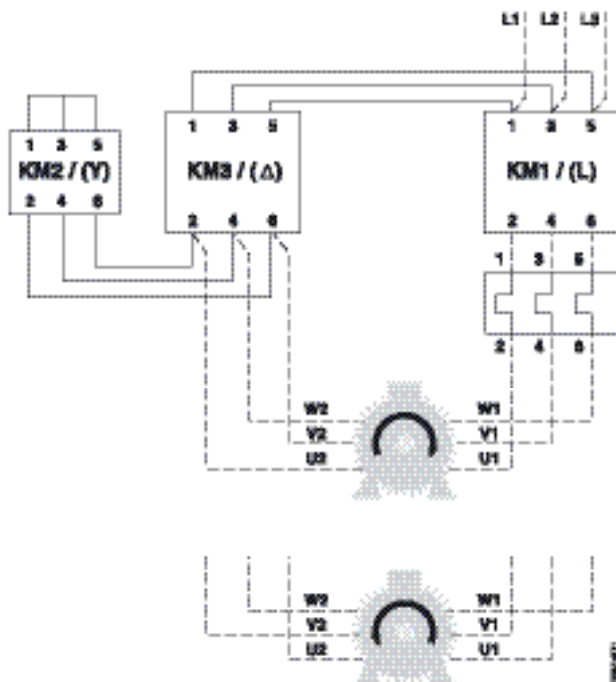
Power circuit diagram A 9 ... AF 750 Contactors
