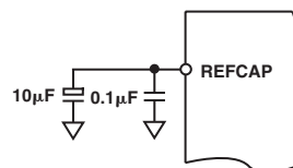
Figure 8. Reference Decoupling
