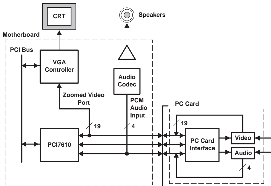
Figure 3–4. Zoomed Video Implementation Using the PCI7610 Controller
