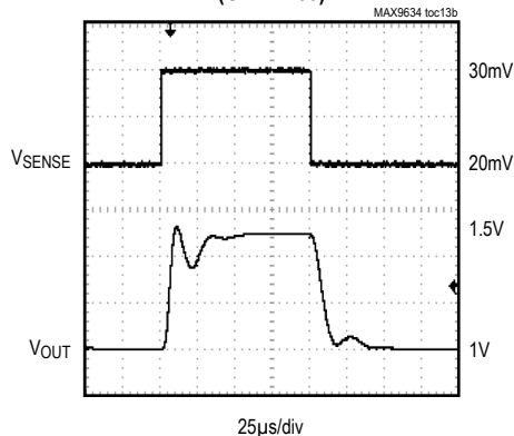
SMALL-SIGNAL PULSE RESPONSE (GAIN = 50)
