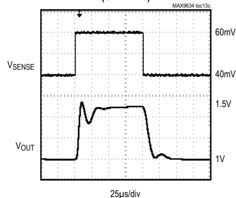
SMALL-SIGNAL PULSE RESPONSE (GAIN = 25)
