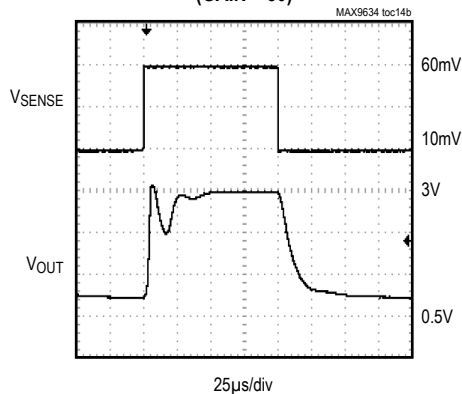
LARGE-SIGNAL PULSE RESPONSE (GAIN = 50)
