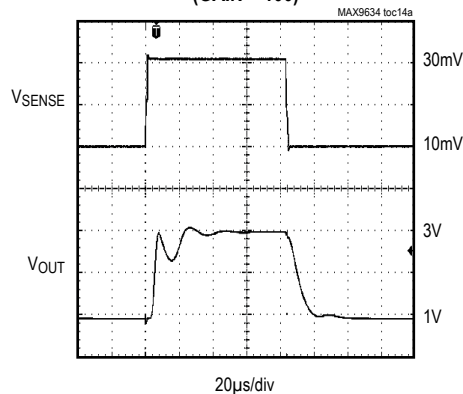
LARGE-SIGNAL PULSE RESPONSE (GAIN = 100)
