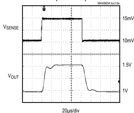
SMALL-SIGNAL PULSE RESPONSE (GAIN = 100)
