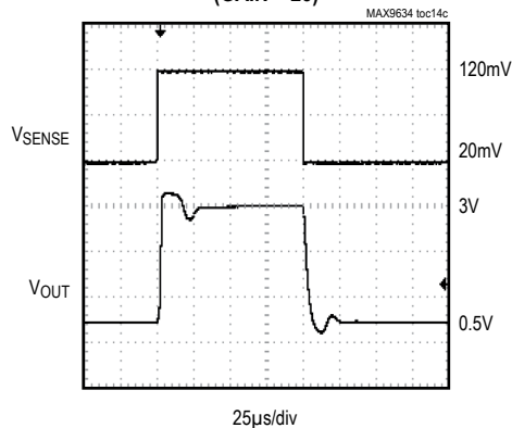
LARGE-SIGNAL PULSE RESPONSE (GAIN = 25)
