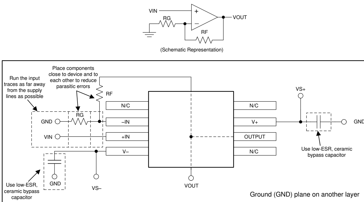
Figure 10-1. Layout Example
