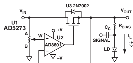
Figure 14. Programmable Booster Voltage Source
