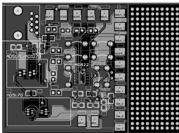
Figure 25. Evaluation Board
