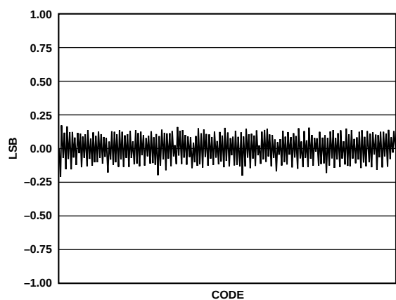
Figure 17. Differential Nonlinearity
