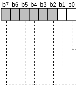
ROM correction enable register (RCR) [Address 020E 16]
