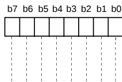
Clock frequency set register(CFS) [Address 0210 16 ]
