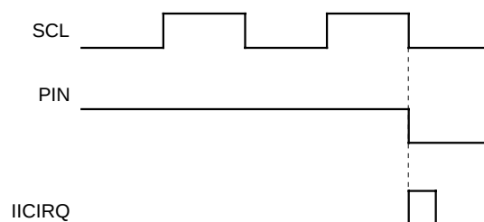
Fig. 8.6.9 Interrupt Request Signal Generation Timing
