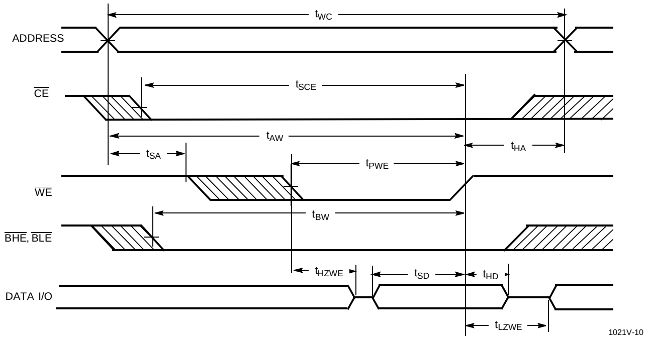
Write Cycle No. 3 ( \overline{\text{WE}} Controlled, LOW)
