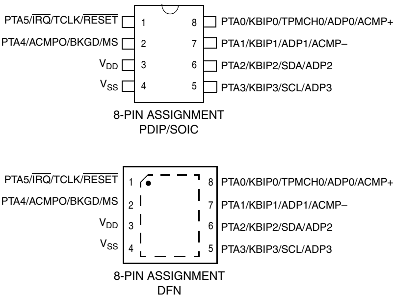
Figure 2-1. 8-Pin Packages
