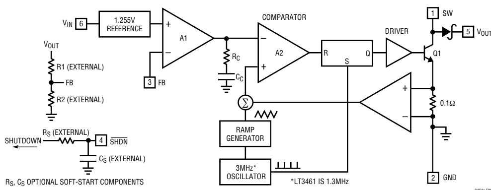
Figure 1. Block Diagram
