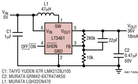
5V to 36V Step-Up Converter (LT3461)
