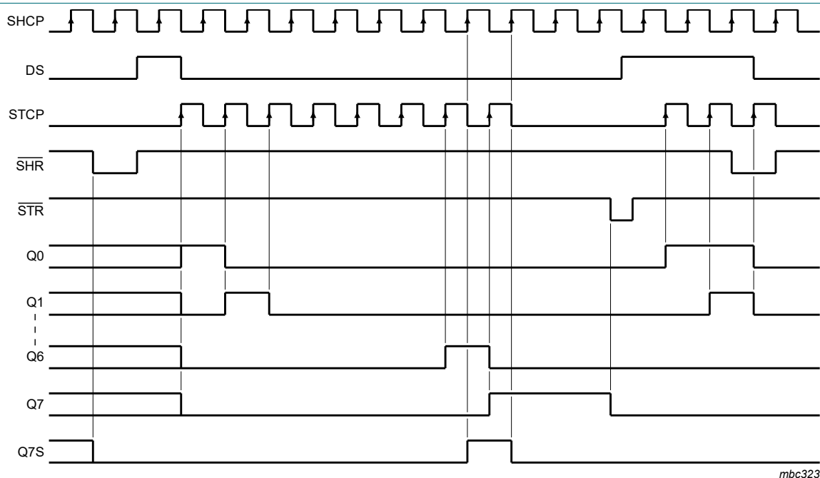
Fig. 5. Timing diagram
