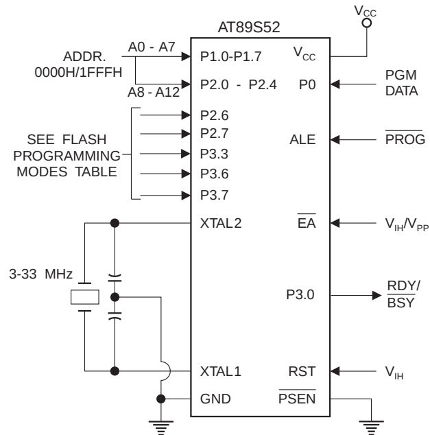
Figure 9. Programming the Flash Memory (Parallel Mode)
