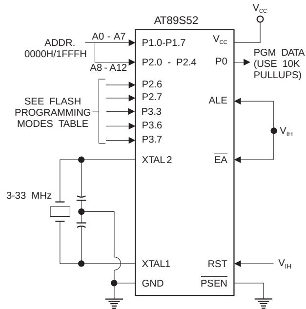
Figure 10. Verifying the Flash Memory (Parallel Mode)
