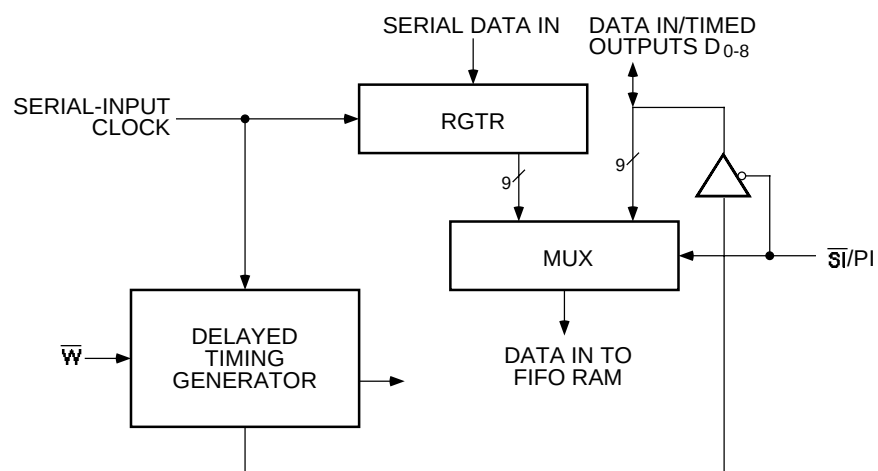
Figure 33. Serial-Input Circuitry
