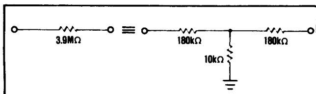
FIGURE 3. Equivalent Resistances.
