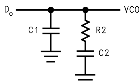
Figure 24. Passive Loop Filter
