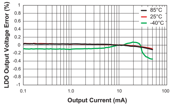
LDO Output Voltage Accuracy vs. Output Current ( V_{IN} = 5.5\text{V} )
