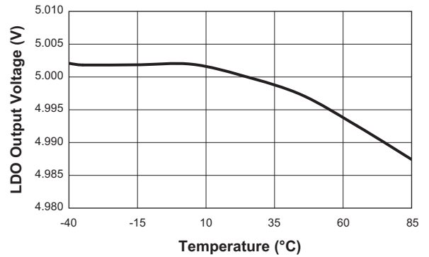
LDO Output Voltage vs. Temperature ( I_{OUT} = 10\text{mA} )
