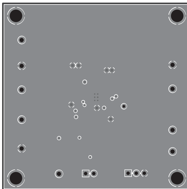
Figure 6: AAT3698-1/-2 Evaluation Board Mid1 Layer Layout.
