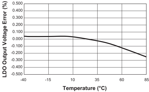
LDO Output Voltage Accuracy vs. Temperature ( I_{OUT} = 10\text{mA} )
