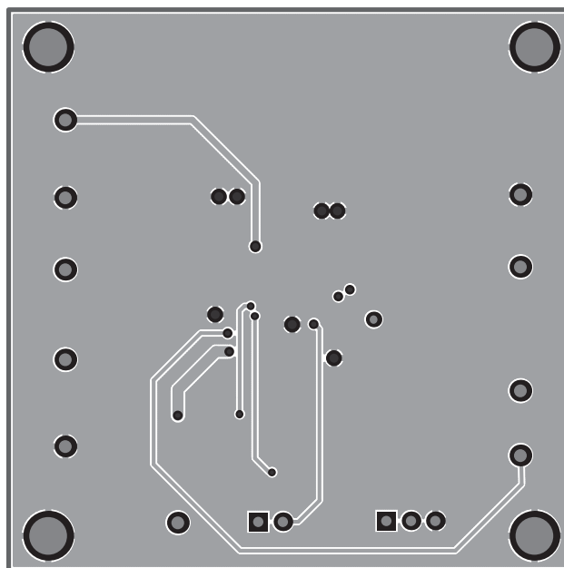
Figure 8: AAT3698-1/-2 Evaluation Board Bottom Side Layout.
