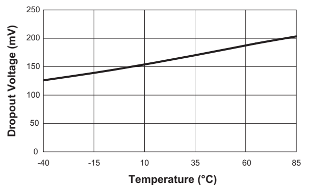
Dropout Voltage vs. Temperature ( I_{OUT} = 30\text{mA} )
