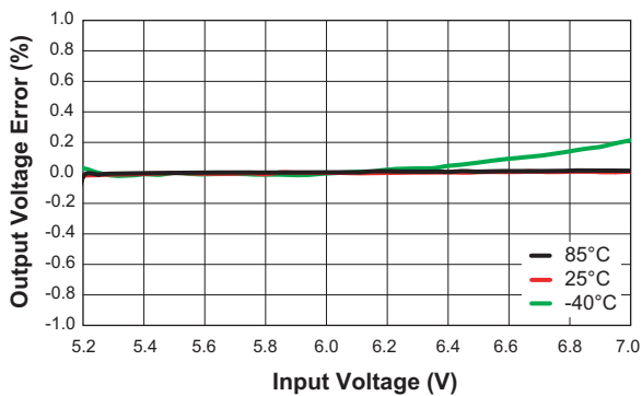
LDO Output Voltage Accuracy vs. Input Voltage ( I_{OUT} = 30\text{mA} )
