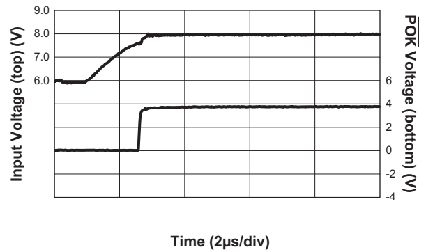
POK ON Delay Time ( R_{LOAD} = 100\Omega )
