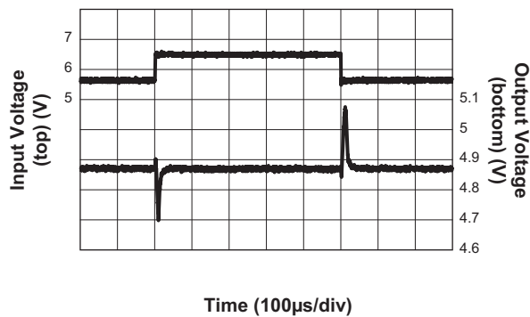
LDO Line Transient
