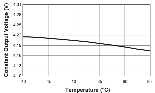
Constant Output Voltage vs. Temperature ( R_{SET} = 3.16K\Omega ; I_{CH\_CC} = 500mA )
