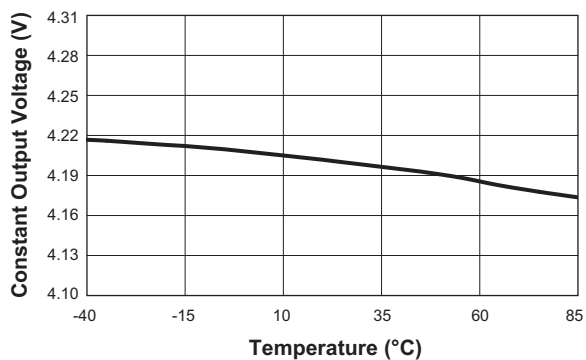
Constant Output Voltage vs. Temperature ( R_{SET} = 1.58K\Omega ; I_{CH\_CC} = 1000mA )
