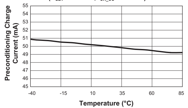
Preconditioning Charge Current vs. Temperature ( R_{SET} = 3.16K\Omega ; I_{CH\_CC} = 500mA )
