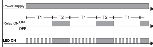
Function Dt - Two state Delay on operate (2xSPDT only)
