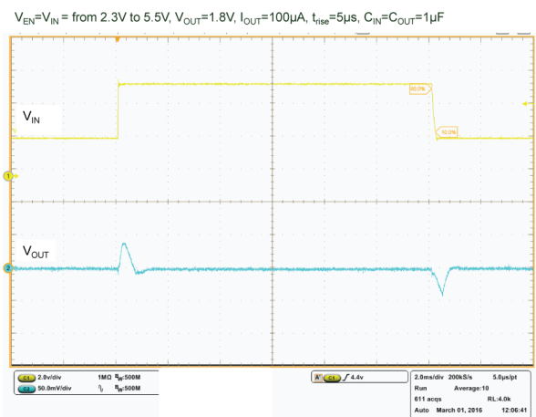
Figure 25. Line transient ( t_{rise} = 5\text{ }\mu\text{s} )
