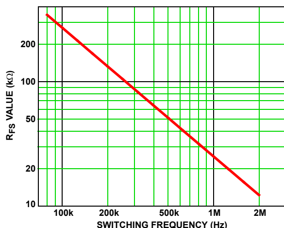
FIGURE 24. R_{FS} vs SWITCHING FREQUENCY
