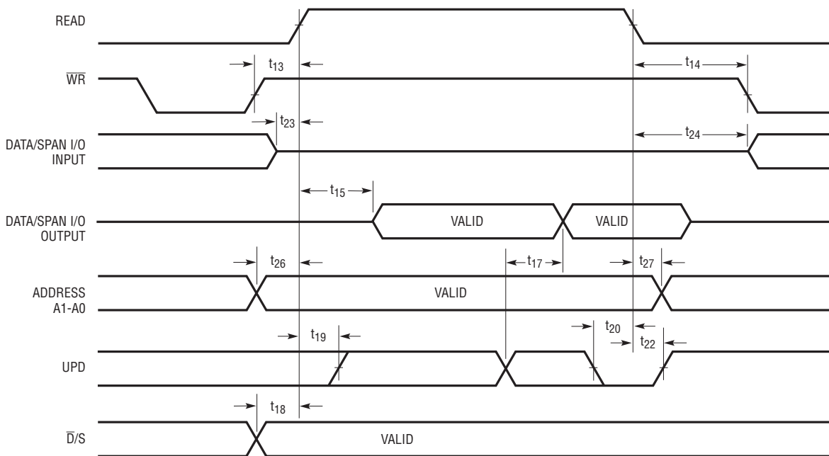
Readback Timing
