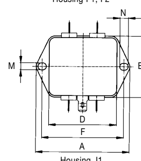
Housing J1
