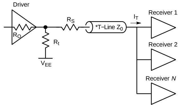
Figure 18. Noise Margin Loss Example
