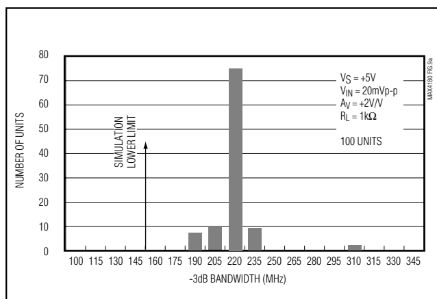
Figure 9a. MAX4180 -3dB Bandwidth Distribution (Single Supply)
