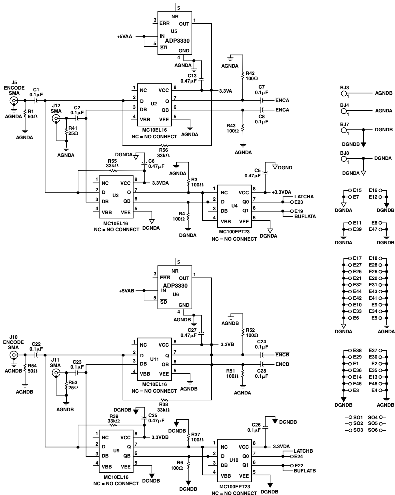
Figure 10c. Evaluation Board
