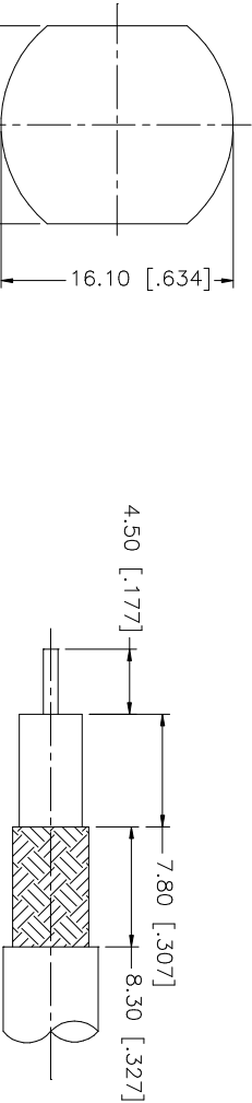
RECOMMENDED CABLE STRIPPING DIMS.
