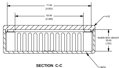
SECTION C-C SCALE 1 : 1
