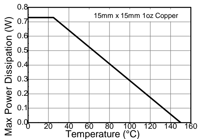
Derating Curve
