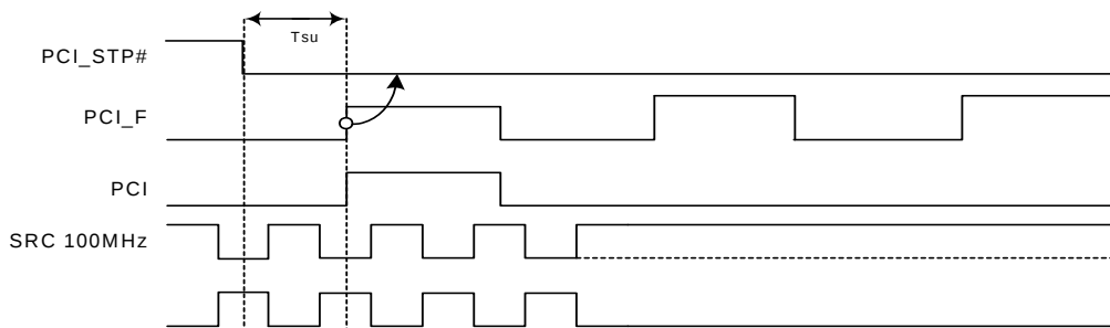
Figure 10. PCI_STOP# Assertion Waveform
