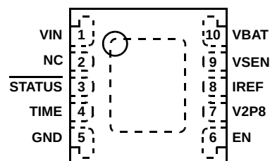
ISL9203A (10 LD 3x3 DFN) TOP VIEW
