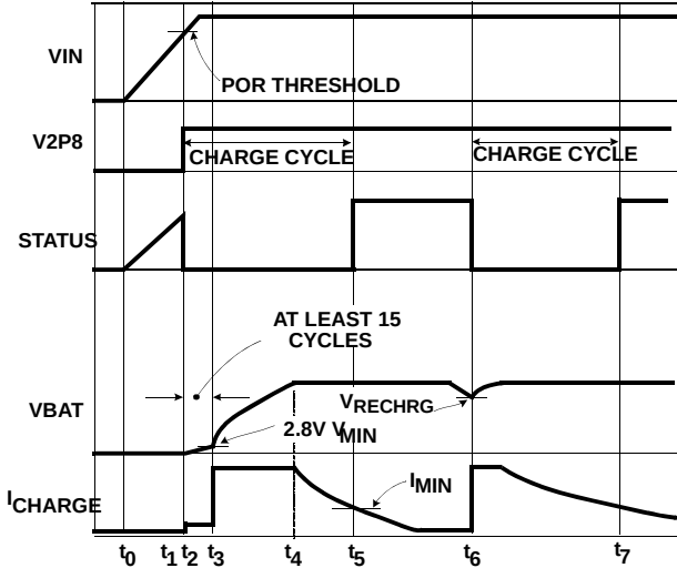
FIGURE 20. OPERATION WAVEFORMS
