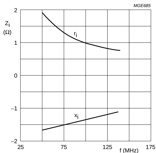
Class-B operation; V_{DS} = 50\text{ V} ; I_{DQ} = 2 \times 0.1\text{ A} ; R_{GS} = 4\text{ }\Omega (per section); P_L = 300\text{ W} . Fig.14 Input impedance as a function of frequency (series components); typical values per section.
