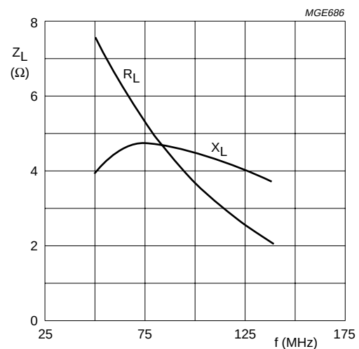
Class-B operation; V_{DS} = 50\text{ V} ; I_{DQ} = 2 \times 0.1\text{ A} ; R_{GS} = 4\text{ }\Omega (per section); P_L = 300\text{ W} . Fig.15 Load impedance as a function of frequency (series components); typical values per section.
