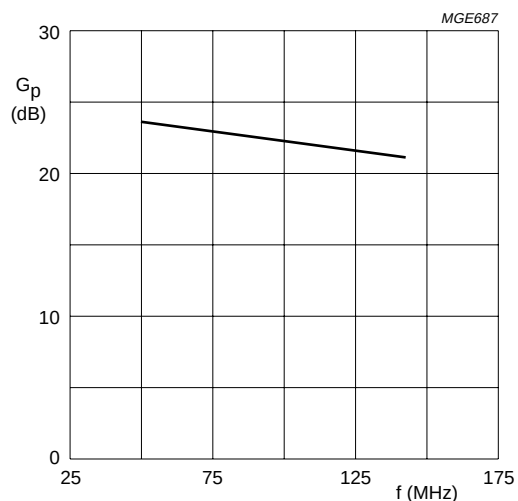
Class-B operation; V_{DS} = 50\text{ V} ; I_{DQ} = 2 \times 0.1\text{ A} ; R_{GS} = 4\text{ }\Omega (per section); P_L = 300\text{ W} . Fig.17 Power gain as a function of frequency; typical values per section.
