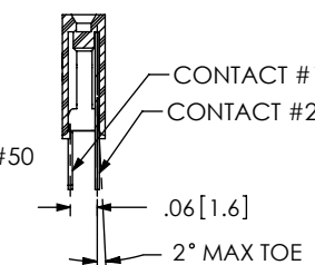
SECTION "B"-"B" BCS-1XX-X-S-DE
