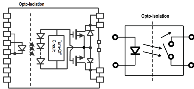
Figure 14 ASSR-601J Equivalent Circuit
