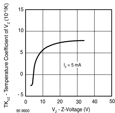
Figure 4. Temperature Coefficient of V_Z vs. Z-Voltage
