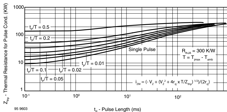
Figure 10. Thermal Response
