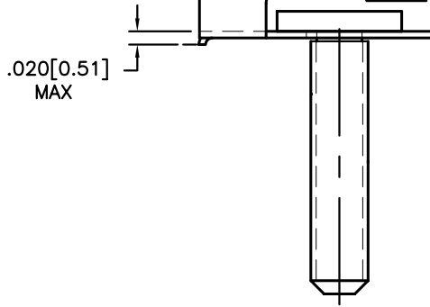
AUX. VIEW "A" TERMINAL w/o TAIL
