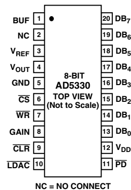
AD5330 PIN CONFIGURATION
