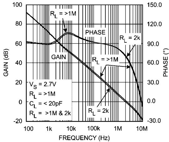
Open Loop Gain and Phase vs. R_L @ 2.7V
