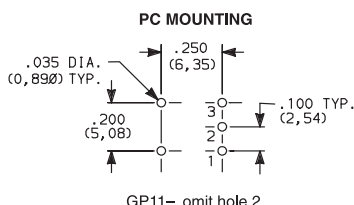
GP11MABE SPST
